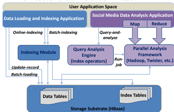
Figure 2. IndexedHBase Architecture.
