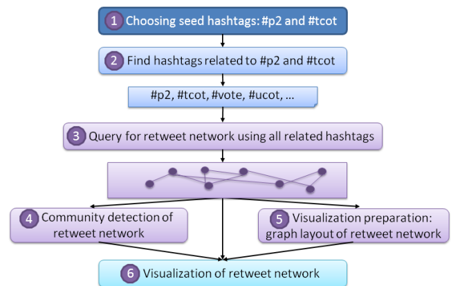
Figure 5. End-to-end analysis workflow in [9].
